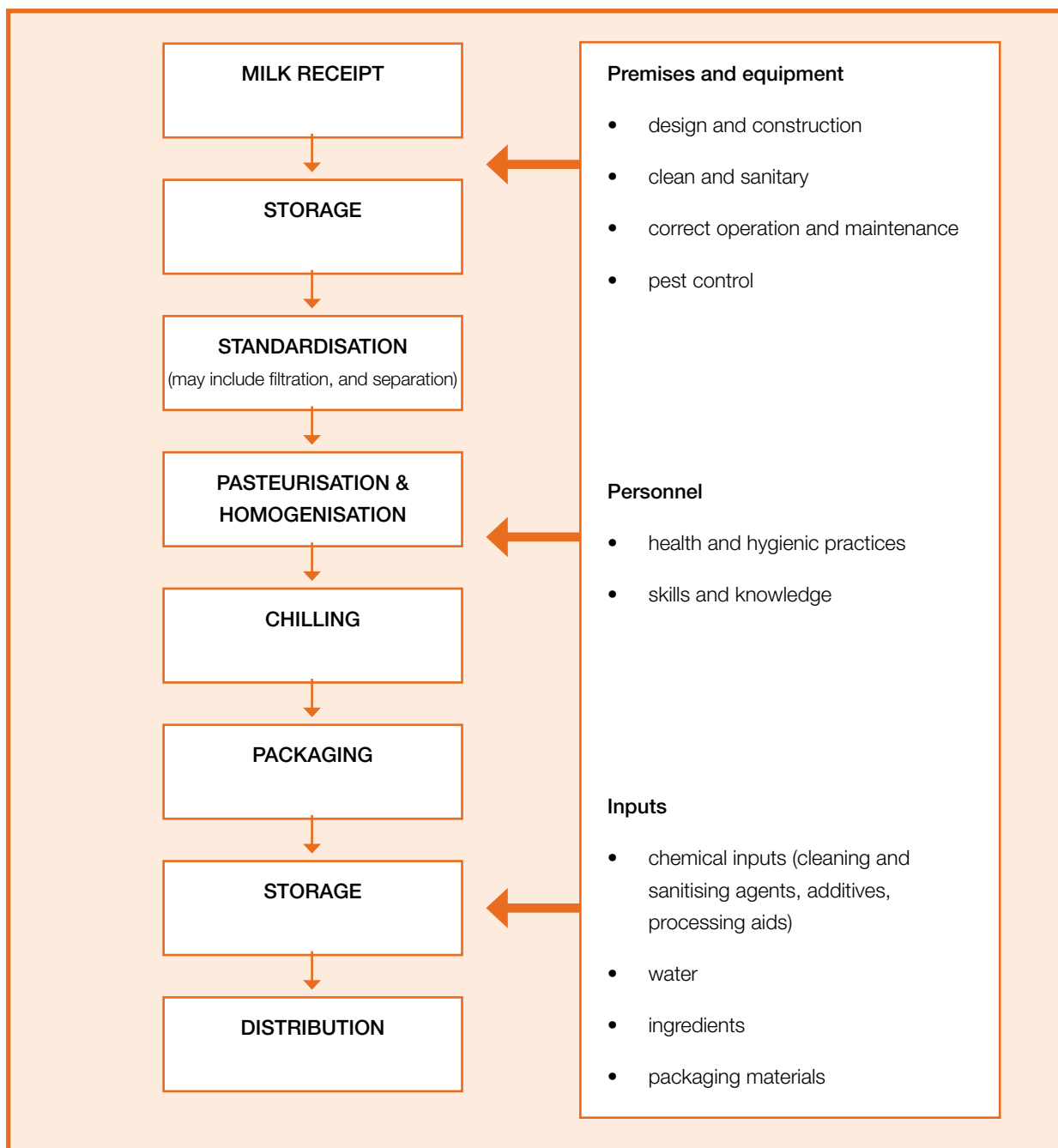
Figure 1: Key steps involved in packaged milk processing
